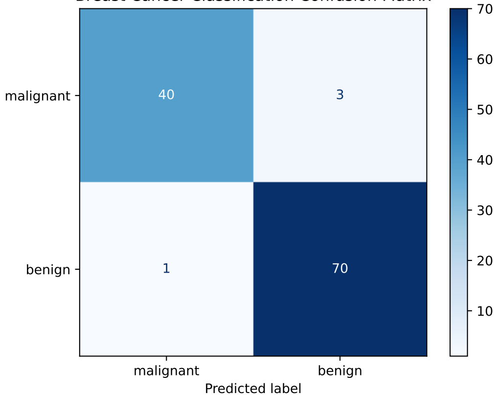
Breast Cancer Classification Confusion Matrix
